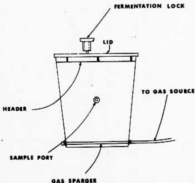
Fig. 1. Carbonation vessel for testing bloater susceptibility of cucumber lines and cultivars to bloater damage.
